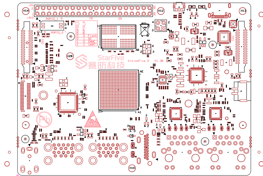
RV002_V1_3B SILKSCREEN TOP RV002_V1_3B OUTLINE
